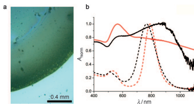
Figure 3. a) Photograph of a partial view of the ring formed upon drop casting of a NR colloid, which was acquired in reflection mode under white-light illumination. b) UV/Vis/NIR spectra of Gem1-NR (red) and CTAB-NR (black) isotropic solutions in water (dashed lines) and their corresponding assemblies onto ITO-coated glass (solid lines). The Gem1-NR array profile reflects the high order of standing NRs and the anisotropic nature of the surface. Note that Gem1-NRs show a significantly narrower LSP band than CTAB-NRs in aqueous isotropic solutions.
